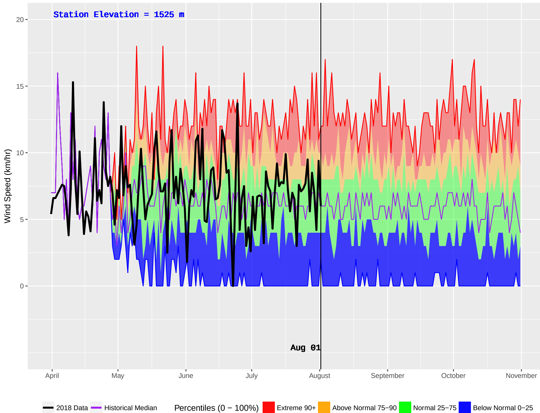
HARBOUR LAKE (250) : Historical (1989–2016) and Current (2018) Daily Wind Speed
