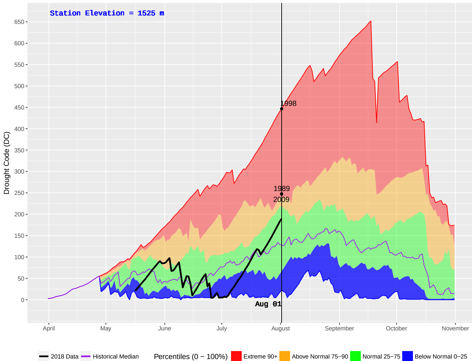
HARBOUR LAKE (250) : Historical (1989–2016) and Current (2018) Daily Drought Code (DC)
