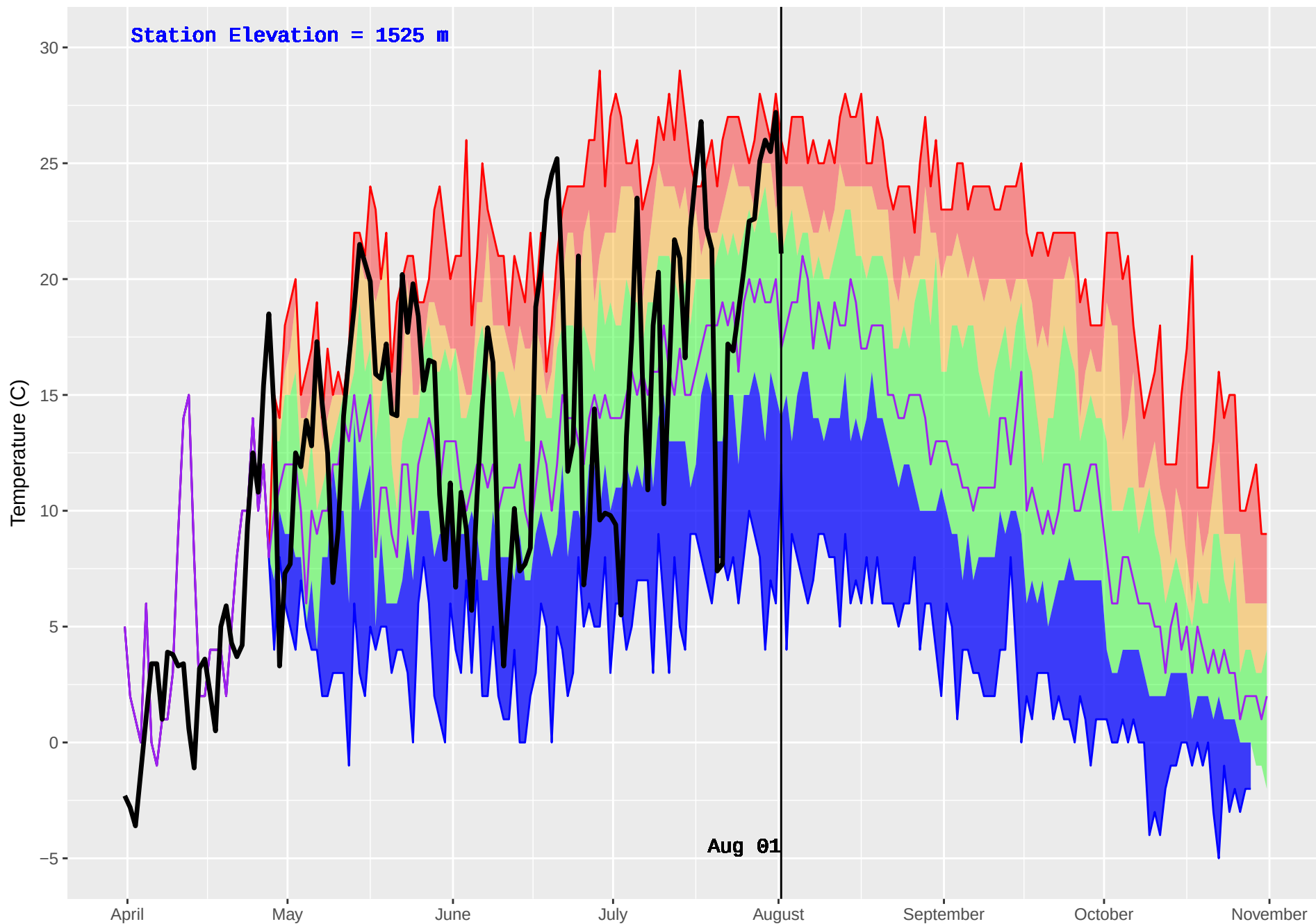
HARBOUR LAKE (250) : Historical (1989–2016) and Current (2018) Daily Temperature
