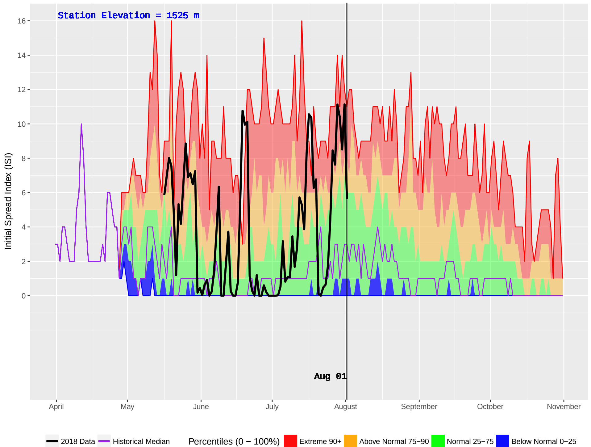
HARBOUR LAKE (250) : Historical (1989–2016) and Current (2018) Daily Initial Spread Index (ISI)
