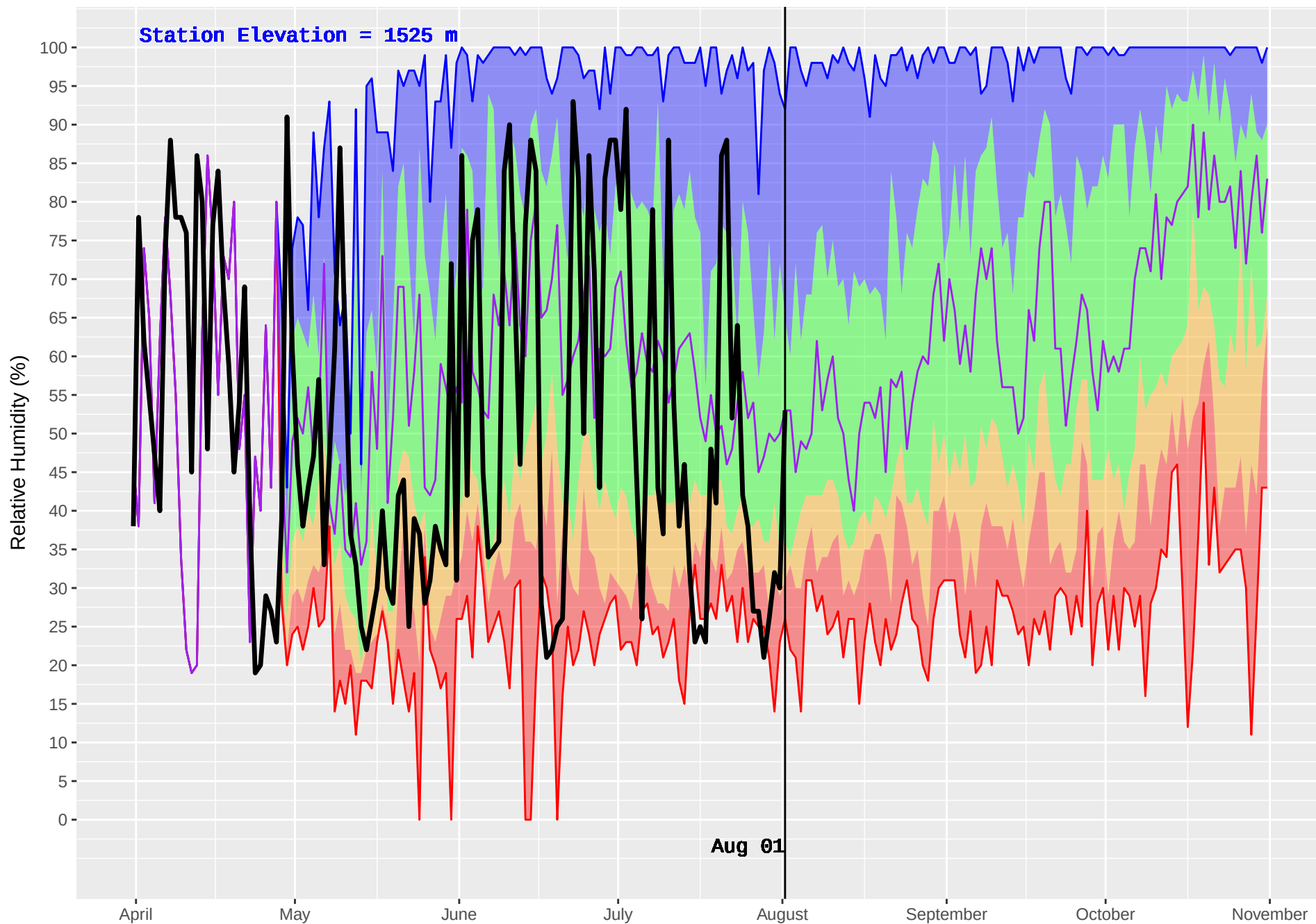
HARBOUR LAKE (250) : Historical (1989–2016) and Current (2018) Daily Relative Humidity
